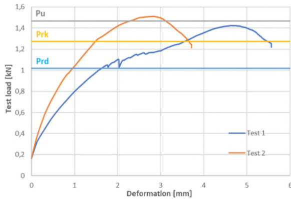
Fig. 5 Test records and statistical evaluation of design values of the shear capacity
