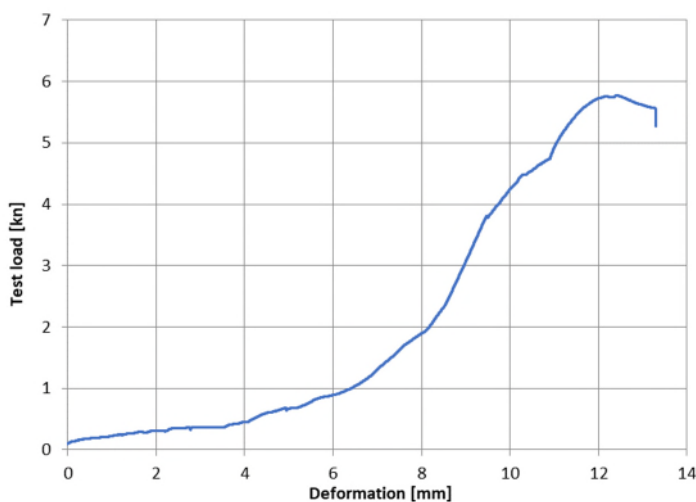
Fig. 6 Test record of the pressure test
