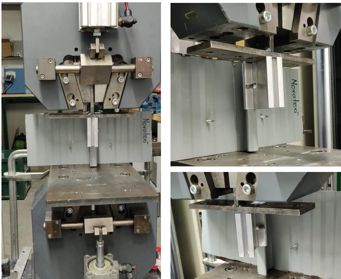
Figure 3 Test set-up for the shear tests
