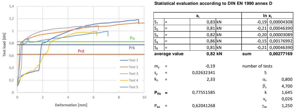
Fig. 4 Test records and statistical evaluation of design values of the shear capacity
